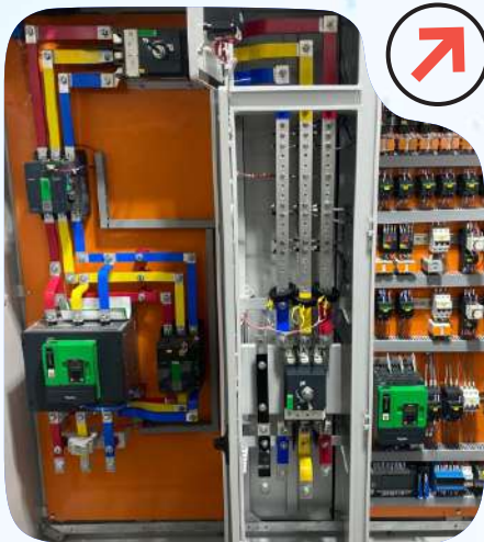
Soft Starter Panel
